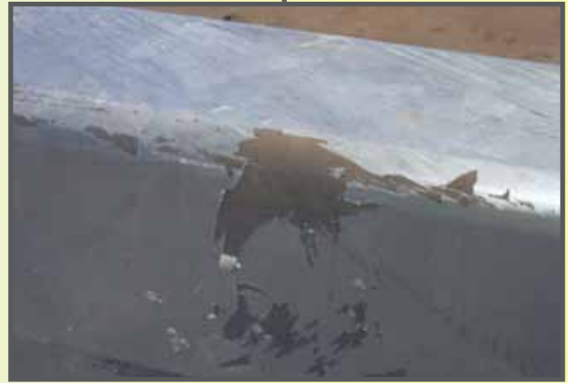
FIGURE 16: DELAMINATION (ACCEPTABLE IF MINIMUM THICKNESS LEVELS ARE MET)
