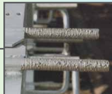
FIGURE 15B: CLOGGED THREADS (ACCEPTABLE AFTER THREADS ARE CLEANED)
