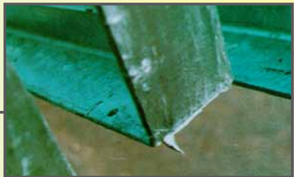
FIGURE 18: DRAINAGE SPIKES
