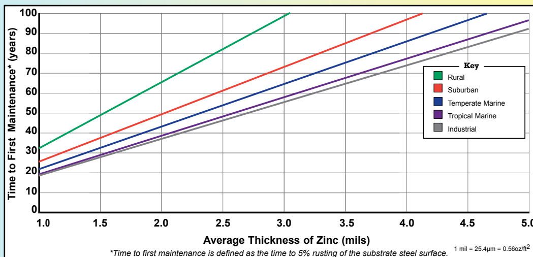
FIGURE 1: TIME TO FIRST MAINTENANCE OF HOT-DIP GALVANIZED COATINGS
