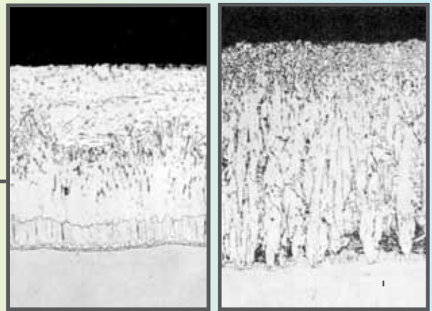
FIGURE 7: RECOMMENDED SILICON VS REACTIVE STEEL
