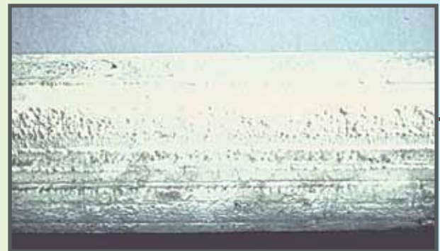
FIGURE 8: ROUGH COATING DUE TO PHOSPHOROUS LEVELS OVER 0.04% (ACCEPTABLE UNLESS HANDRAIL)
