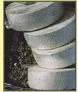
FIGURE 26: ROUGH SURFACE CONDITION/ STEEL SURFACE CONDITION (ACCEPTABLE)
