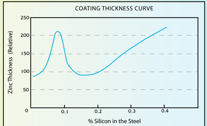
FIGURE 6: SANDELIN CURVE
